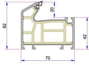
Penwood 760 Kasa Profili P.A.706.1000.600.2.BC.01
