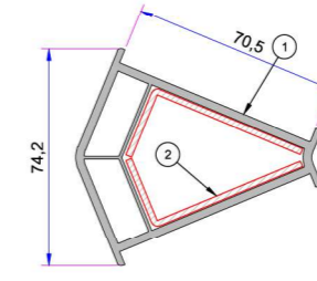
1. 135° Köşe Profili P.A.070.5102.600.0.00.19 2. Destek Sacı (25x55) 1,2mm - 34022 - 12303 1,5mm - 34022 - 15303 2 mm - 34022 - 20303
