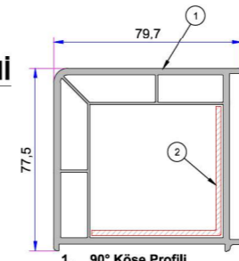
1. 90° Köşe Profili P.A.070.5100.600.0.00.19 2. Destek Sacı (55x55) 1,2mm - 34022 - 12305 1,5mm - 34022 - 15305 2 mm - 34022 - 20305
