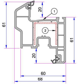
1. Damlalıklı Kanat Profili P.A.632.2200.600.0.BC.01 2. Destek Sacı (29x30x29) 1,2mm 34022-12002 1,5mm 34022-15002 2 mm 34022-20002
