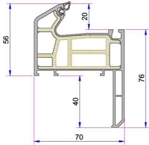
Penwood 760 Pervazlı Kasa Profili P.A.706.1200.600.2.BC.01
