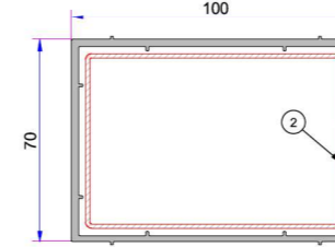
1. Kutu Profili (70x100) P.A.070.5202.600.0.00.19 2. Destek Sacı (60x90) 1,2mm - 34022 - 12121 1,5mm - 34022 - 15121 2 mm - 34022 - 20121
